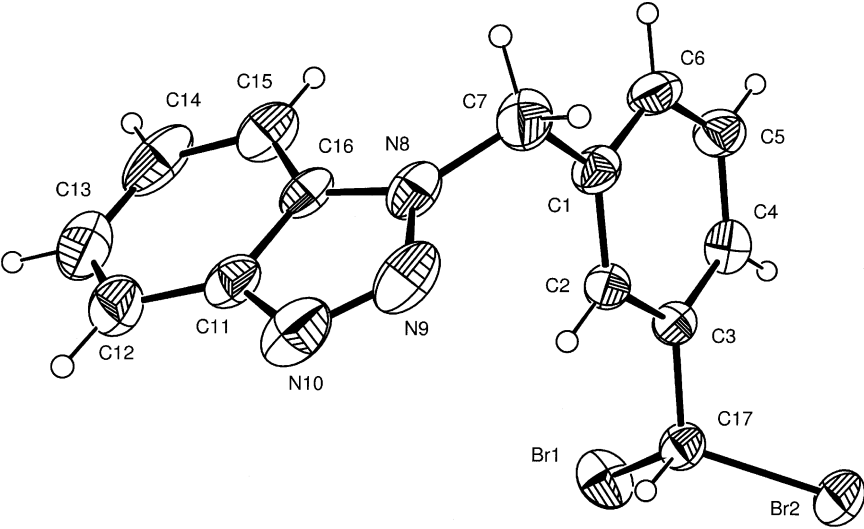
FIGURE 1 ZORTEP plot of the molecule with 30% probability displacement ellipsoids and with atomic numbering scheme.
