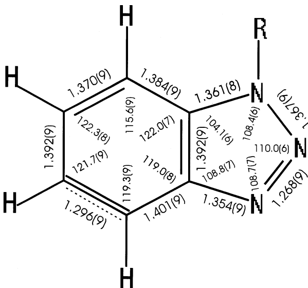
FIGURE 2 Possible delocalized form of the benzotriazole ring in the molecule.
