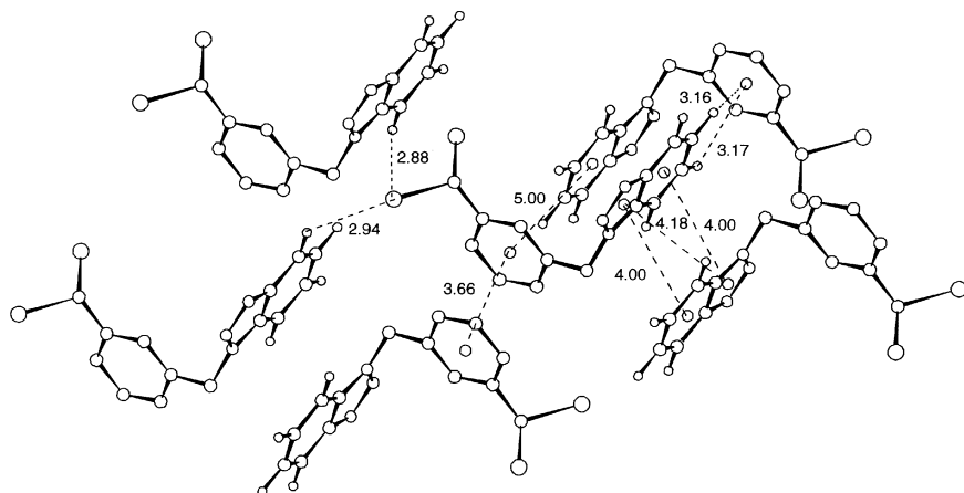
FIGURE 3 Diagram illustrating all possible interactions of the molecule.
