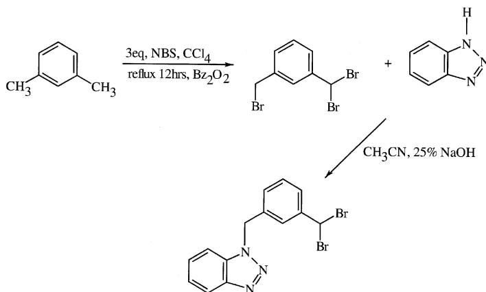
SCHEME 1 Synthetic pathway of the title compound.
