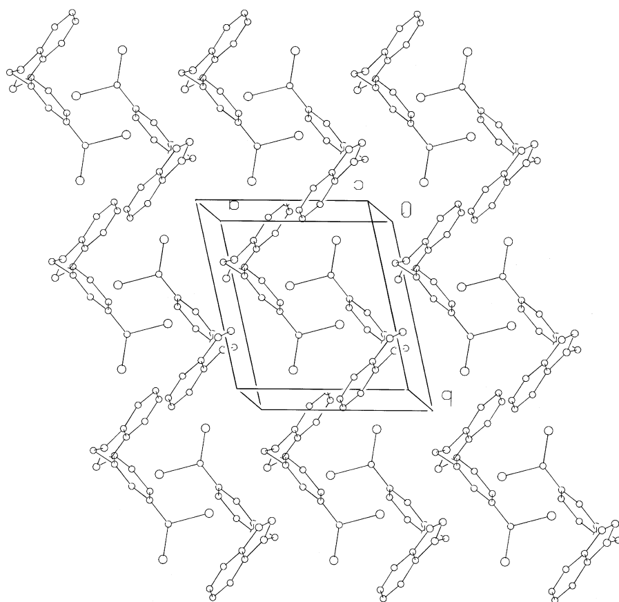
FIGURE 4 Packing of the molecules viewed down c axis.
